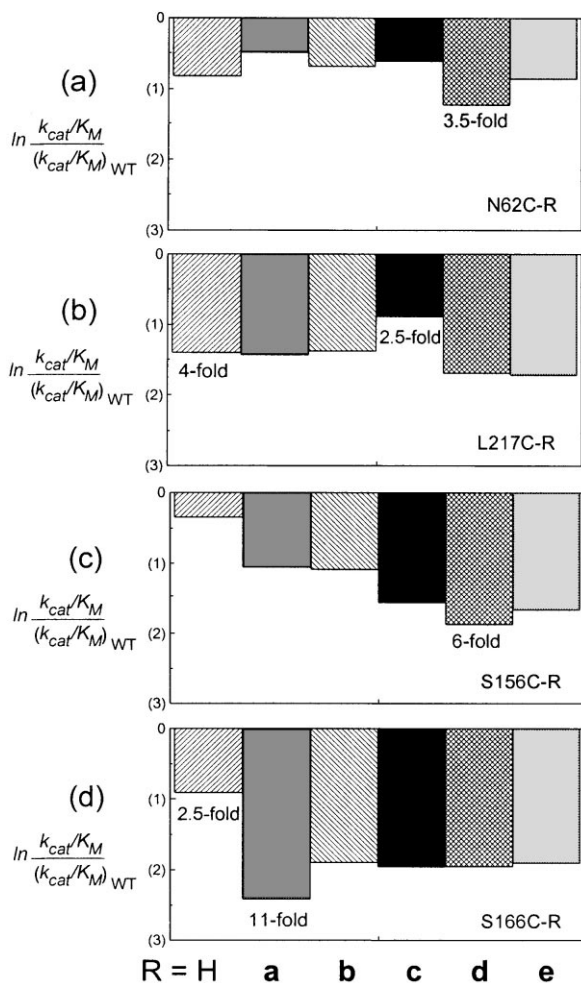
Figure 2. Altered specificity patterns relative to WT as the level of negative charge increases in N62C, L217C, S156C and S166C mutants and CMMs with suc-AAPF-pNA as the substrate: (a) The k_{\text{cat}}/K_M s for N62C CMMs alternate at moderately reduced levels, 1.5- to 3.5-fold lower than WT, which are established by the initial mutation to N62C (R=H). (b) L217C CMMs show steady but lower levels of k_{\text{cat}}/K_M , 4- to 5.5-fold lower than WT, which are again established by the initial mutation to cysteine. The exception is L217C- c which is only 2.5-fold lower than WT, possibly due to favourable binding of substrate to the phenyl ring of the aromatic side chain introduced by modification. (c) From the small reduction caused by mutation to S156C (R=H), k_{\text{cat}}/K_M s decrease monotonically to 6-fold lower than WT for S156C- d . The k_{\text{cat}}/K_M of S156C- e is partially restored. (d) k_{\text{cat}}/K_M decreases only 2.5-fold upon mutation to S166C (R=H) but decreases dramatically to 11-fold lower than WT when the negatively charged sulfonatoethyl side chain a is introduced. In parallel to N62C and L217C CMMs, k_{\text{cat}}/K_M for S166C CMMs does not decrease further to any significant extent as the level of negative charge increases.
