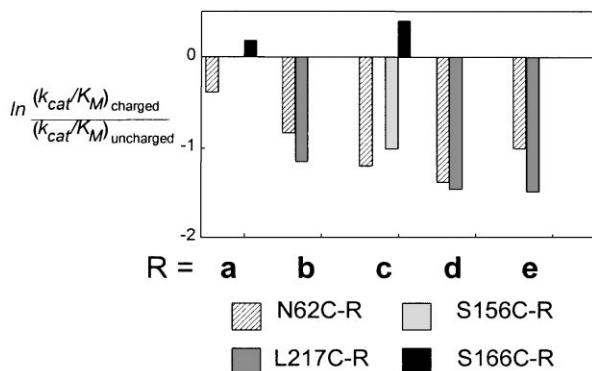
Figure 3. The effects of introducing negative charge to CMMs: \ln(k_{\text{cat}}/K_{\text{M}}) , with suc-AAPF-pNA as the substrate, of the negatively charged N62C, L217C and S156C CMMs decreases relative to that of near-isosteric uncharged CMMs as the level of negative charge increases (from side chain a to e). In contrast, this value for the corresponding S166C CMMs increases with increasing negative charge.
