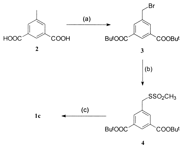
Scheme 2. (a) (i) \text{Im}_2\text{CO} , DMF, 40°C then DBU, t -BuOH, 84%, (ii) NBS, azobis(cyclohexanecarbonitrile), \text{CCl}_4 , \Delta , 96%; (b) \text{NaS-SO}_2\text{CH}_3 , DMF, 50°C, 60%; (c) \text{CF}_3\text{COOH} , \text{CH}_2\text{Cl}_2 , 91%.
